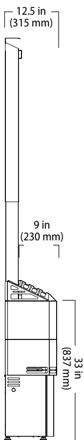
Saunum Air 5kW and 7kW (Closed stone basket)
